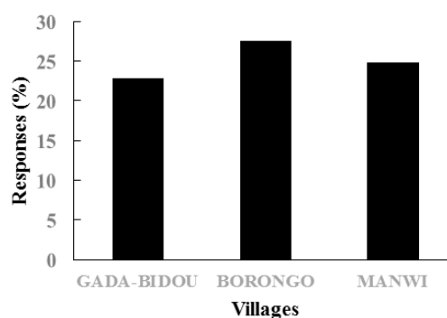
Figure 2. Degree of knowledge of woody species indicators of soil fertility in the three surveyed villages of the Sudano-guinea savannahs of Ngaoundere, Cameroon.
